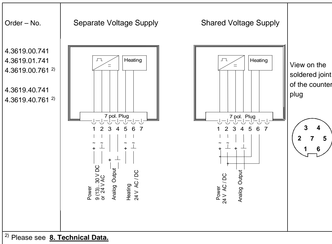
Figure 3: Connecting Diagram for Models with Connector
